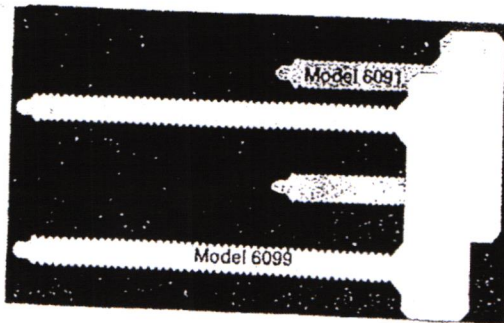
Model 6099 Jumbo Cable Tag, 8" x 2" writing area, with 2 12" straps to pass around conductor up to 6" O.D.
