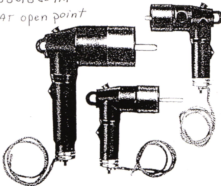
Figure 1. Metal Oxide Elbow Surge Arresters shown from left to right: 35 kV, 25 kV and 15 kV.
