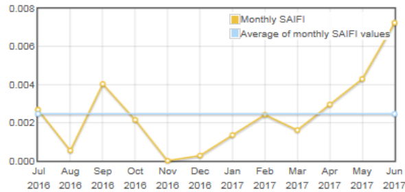
Historical Monthly SAIFI Chart
